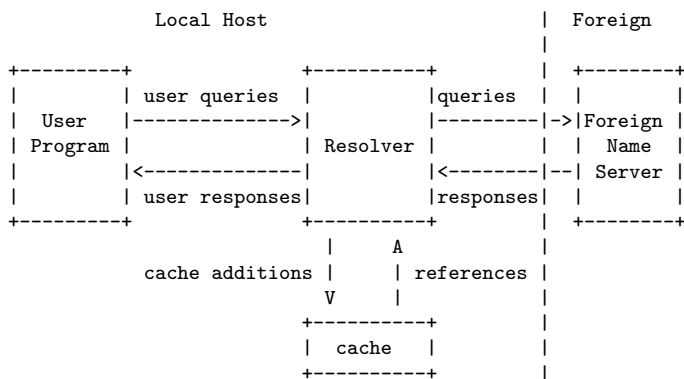
Figura 2.3: DNS (RFC1035).
